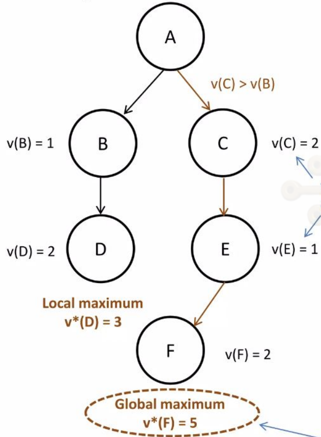
Example of Finding Global Maximum
