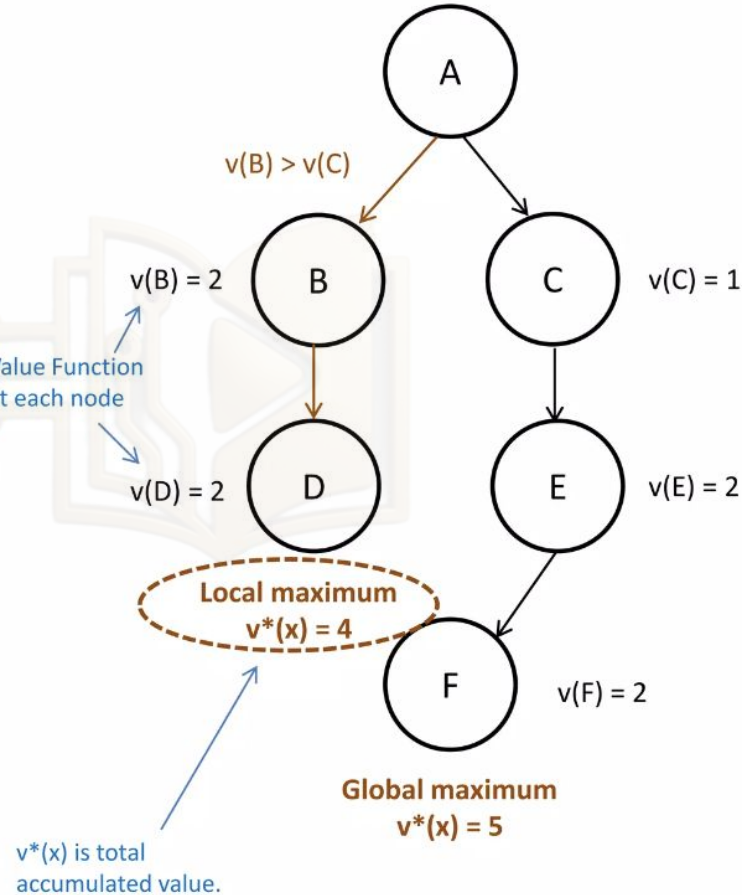
Example of Finding Local Maximum
